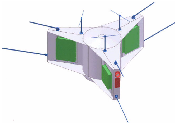
The former and well-known P3-structure of P3A, AO-10 and AO-13 could suit the needs of P3E.
