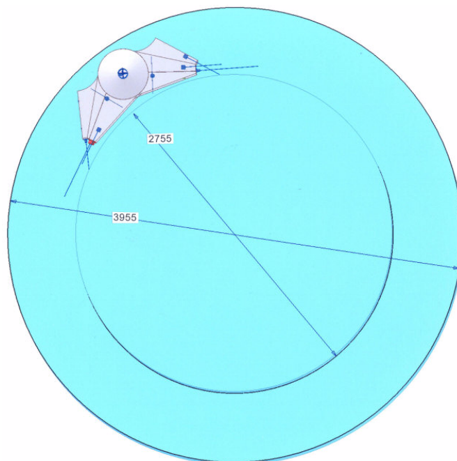
Spacecrafts must fit in between the inner and outer circle of the ASAP-5 spaceframe.
